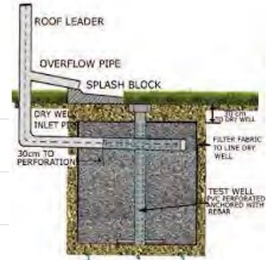
Soak Away Pit
