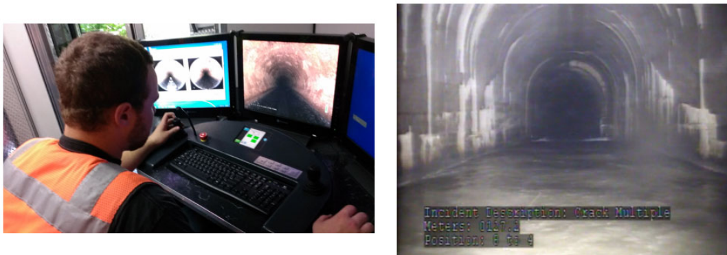
Figure 18 CCTV Inspection
