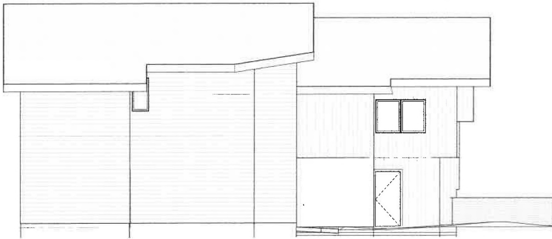
2 SOUTHEAST ELEVATION SCALE: 1/4" = 1'-0"
