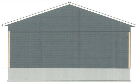
2 Rear Elevation
